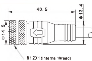
M12 Female, Straight
