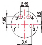
4 Pin Female
